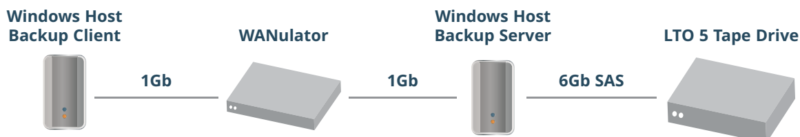
Figure 1: Unaccelerated infrastructure
